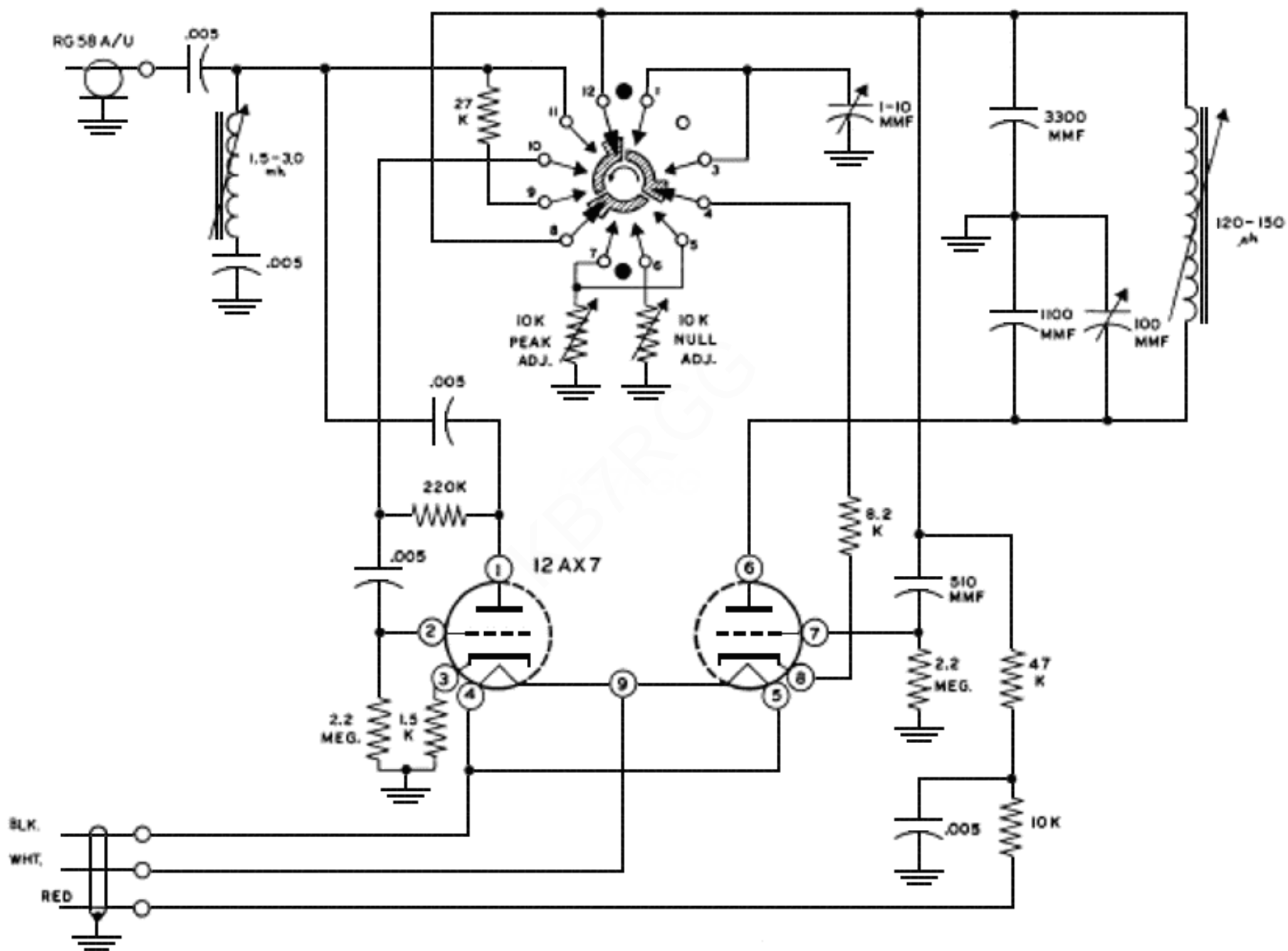
SCHEMATIC OF Q MULTIPLIER QF-1
