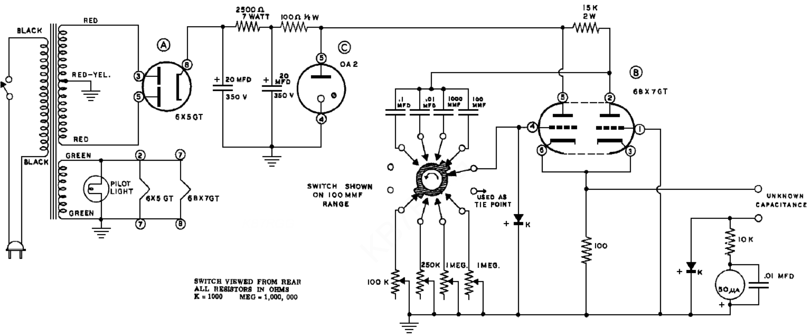
SCHEMATIC HEATHKIT DIRECT READING CAPACITY METER MODEL CM-1
