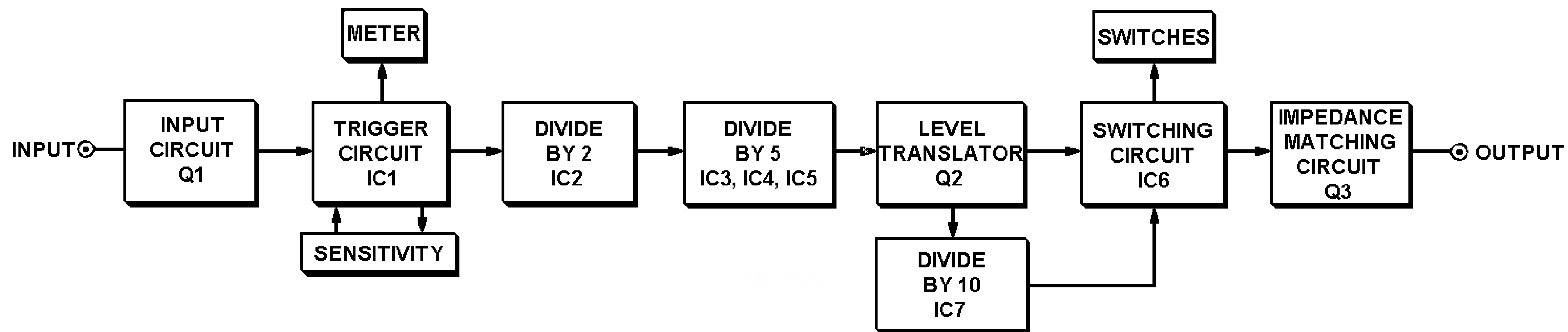
HEATHKIT IB-102 BLOCK DIAGRAM
