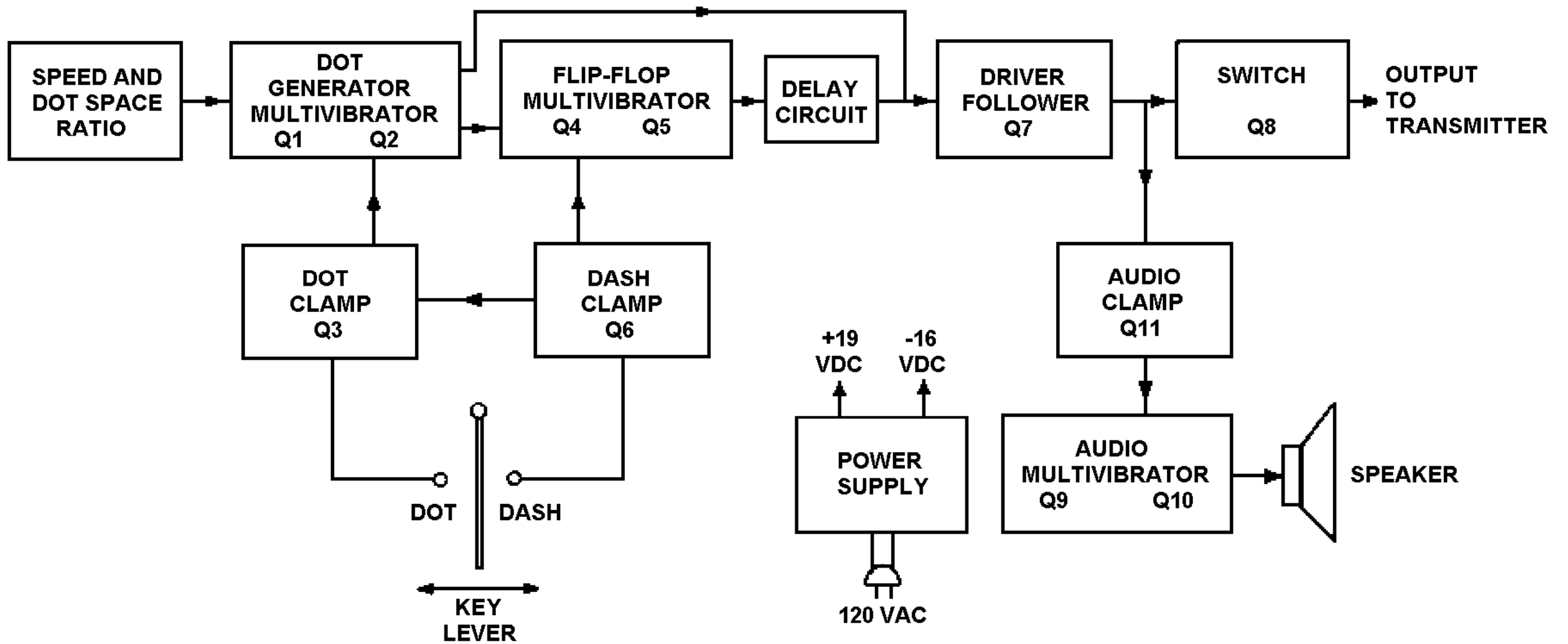
HEATHKIT HD-10 BLOCK DIAGRAM
