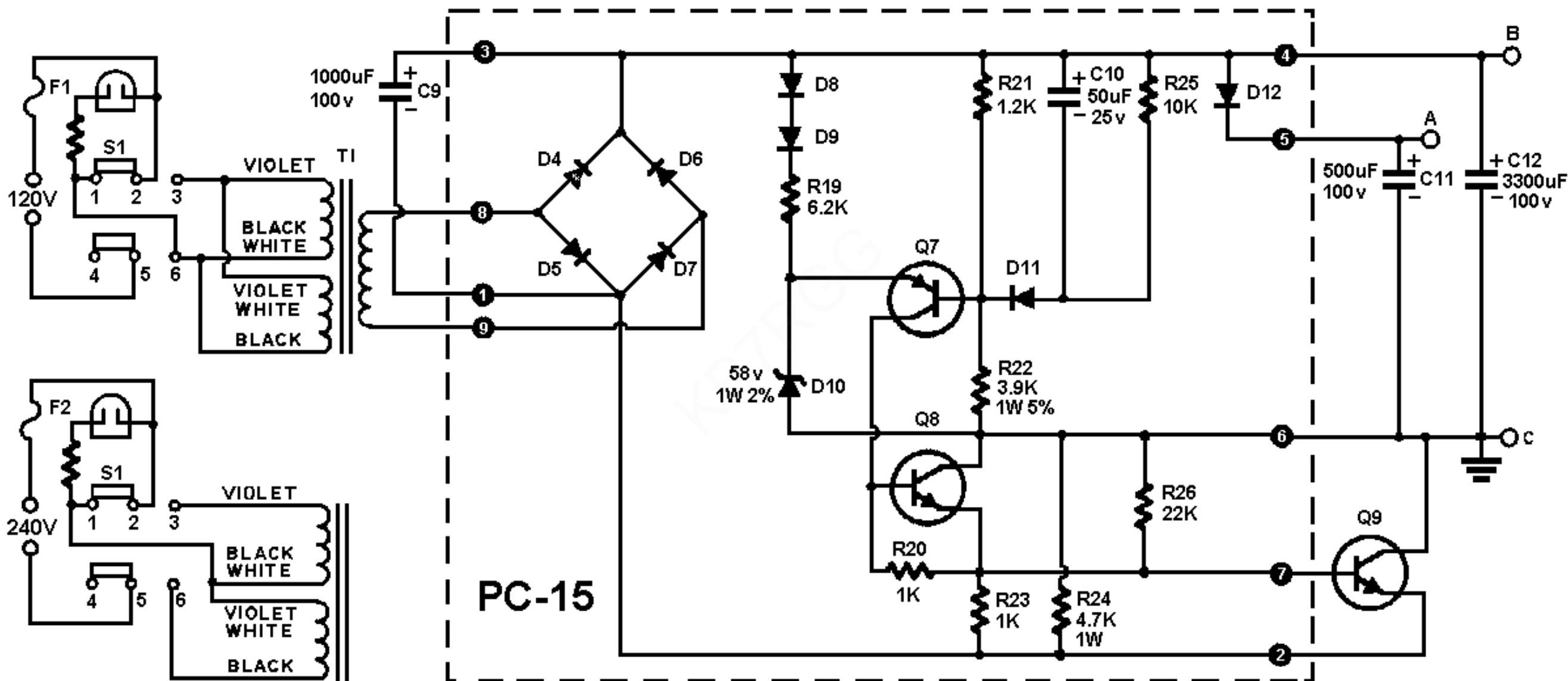
Dynaco Stereo 120 Power Supply
