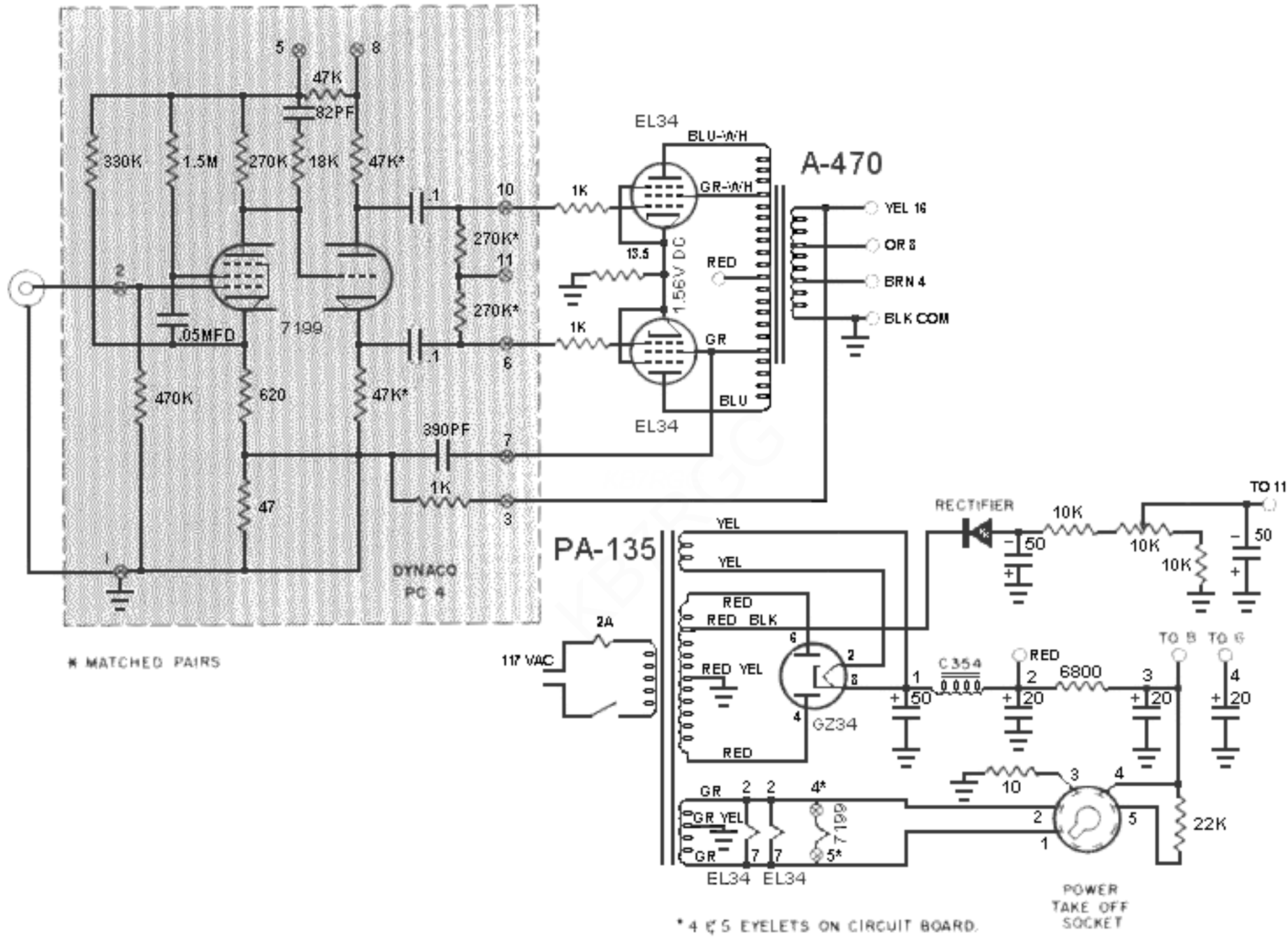
DYNAKIT MARK IV 40 WATT POWER AMPLIFIER
