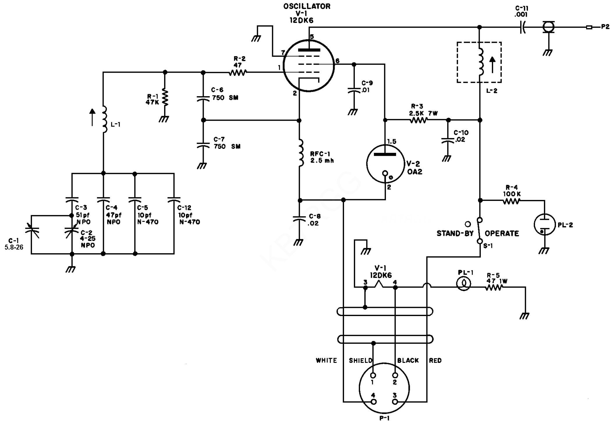
KNIGHT V107 SCHEMATIC DIAGRAM
