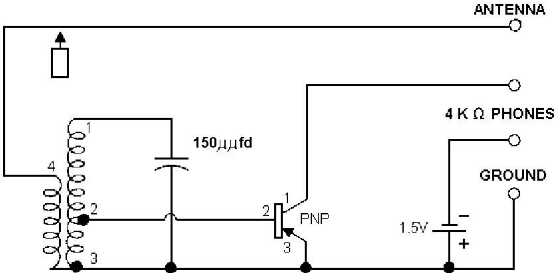
Knight-Kit Trans-Midge Schematic
