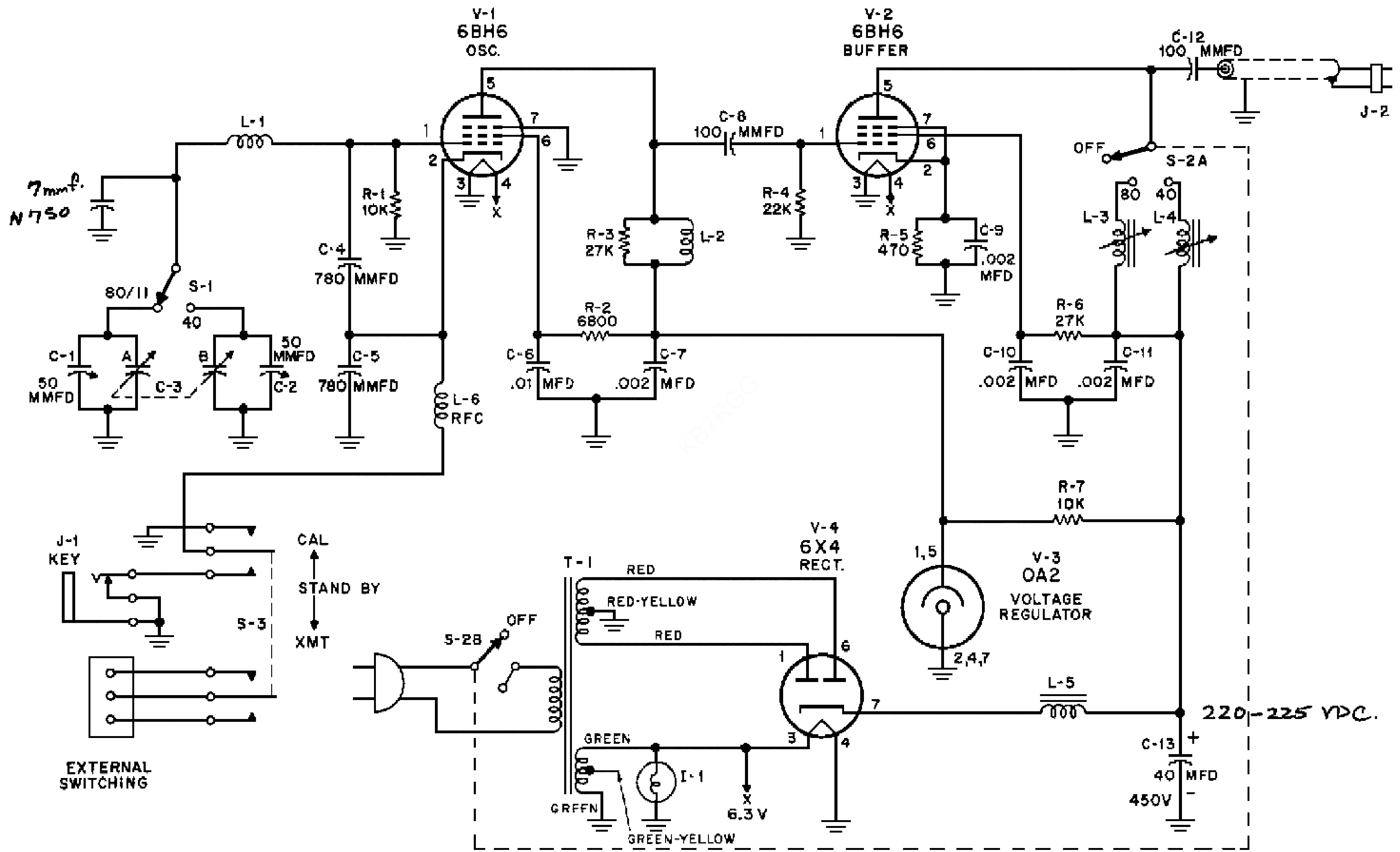
SCHEMATIC DIAGRAM, KNIGHT VFO
